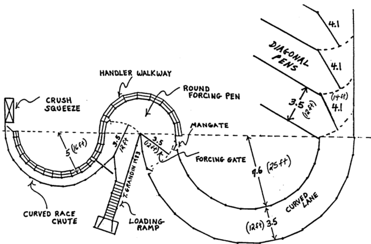
Figure 6. basic Curved Handling Facility.
