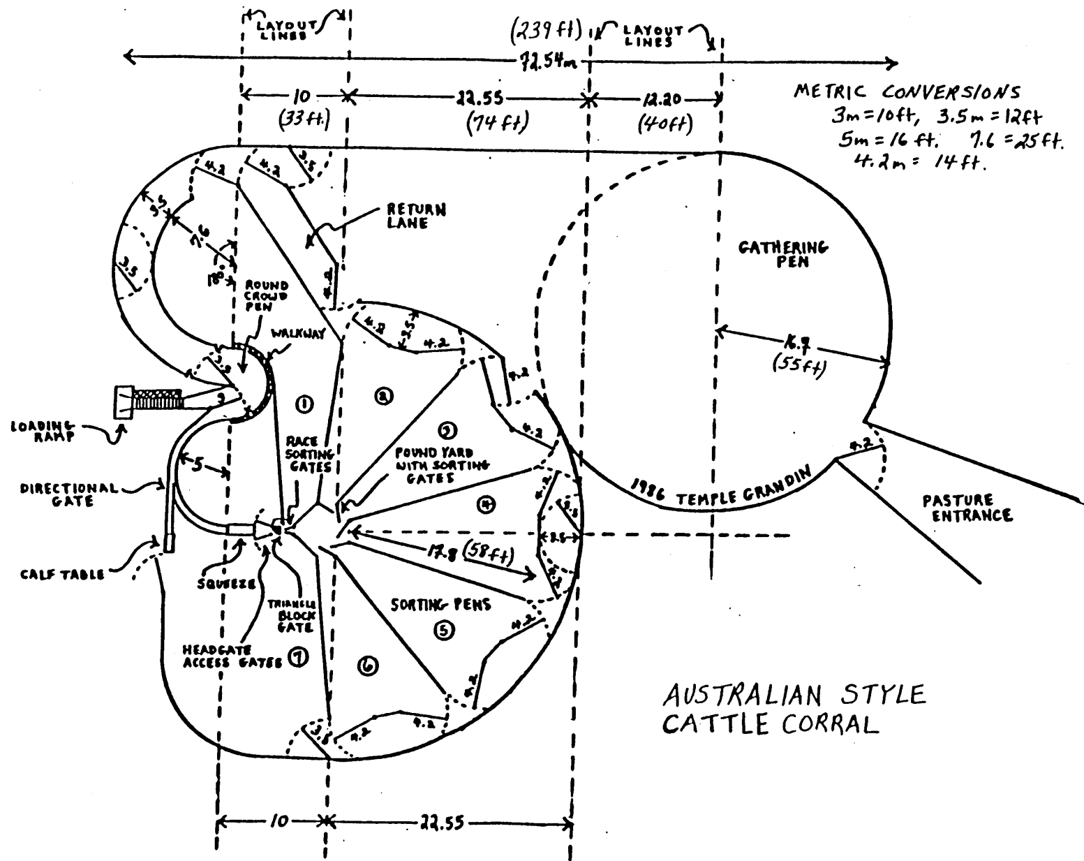
Figure 8. Corral for Sorting and Individual Evaluation of Cattle. Can be Used with Electronic Sorting Systems.
